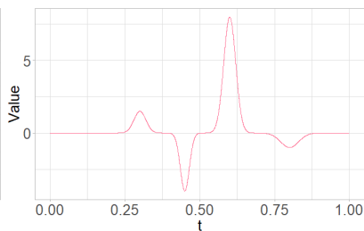
f_2(t) , bumpy function
