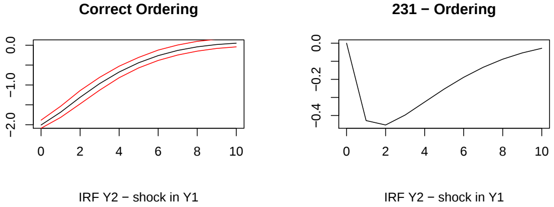
Figure 3: Comparison of two IRFs from different Permutations
