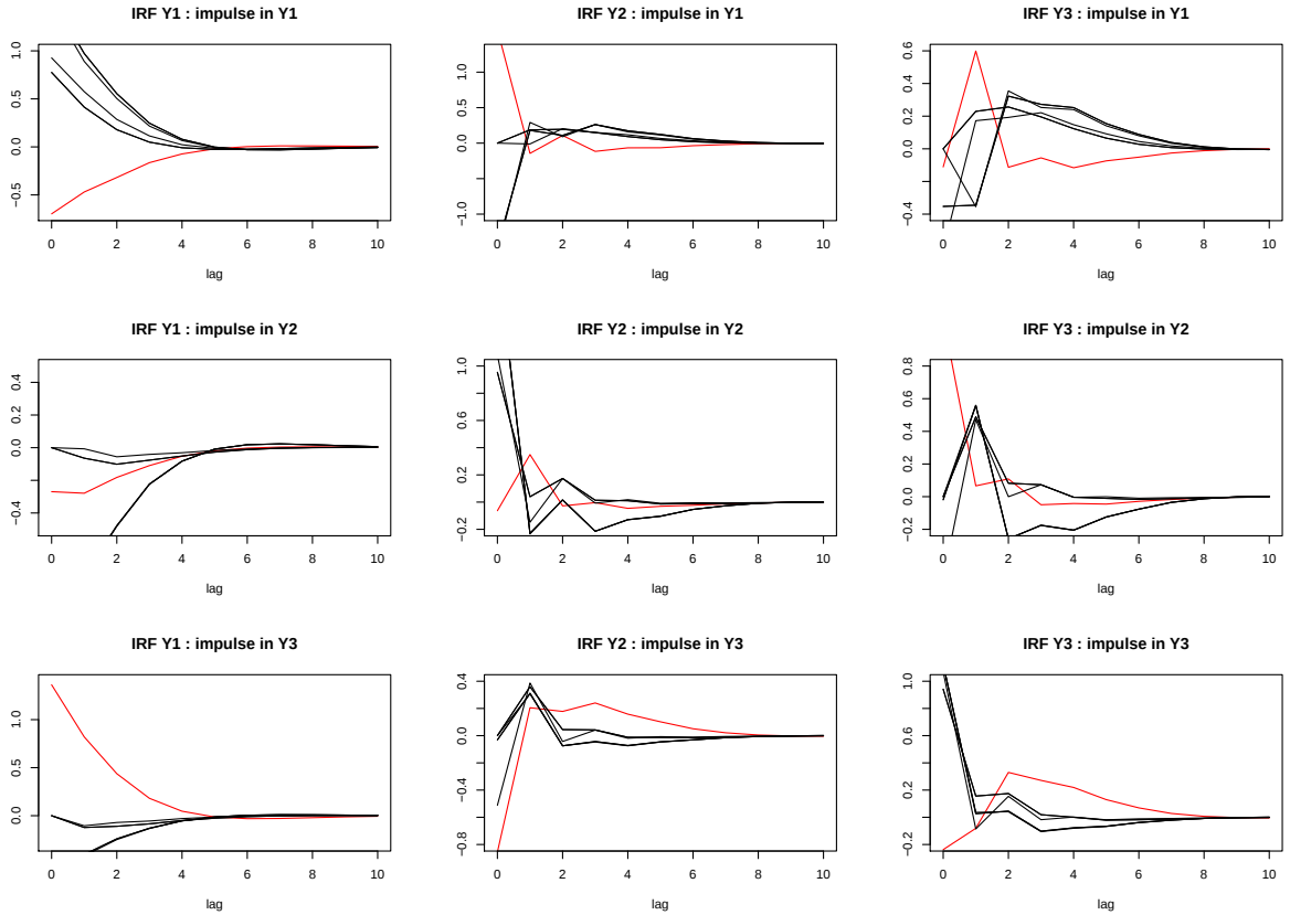
Figure 7: Comparison of impulse responses for different permutations
