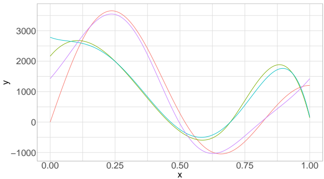
Figure 21: FPC Regression, 4 harmonics - f_1, Y_1
