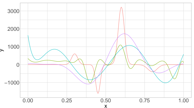
Figure 24: FPC Regression, 4 harmonics - f_2, Y_2
