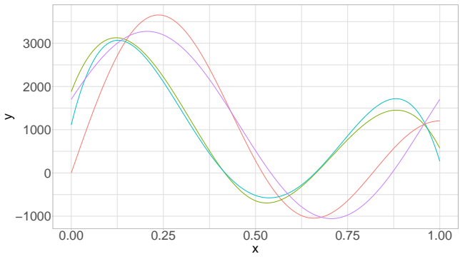
Figure 17: FPC Regression, 3 harmonics - f_1, Y_1
