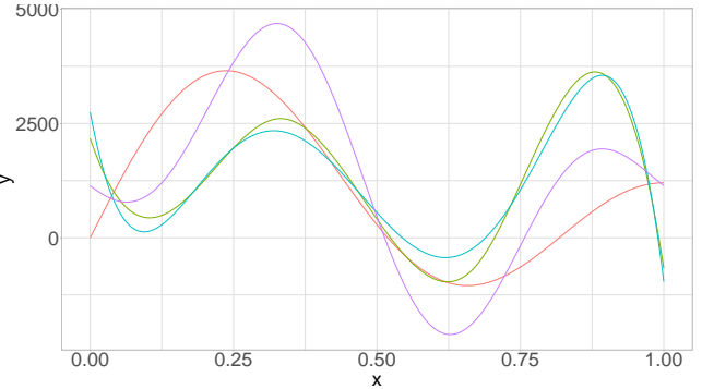
Figure 22: FPC Regression, 4 harmonics - f_1, Y_2
