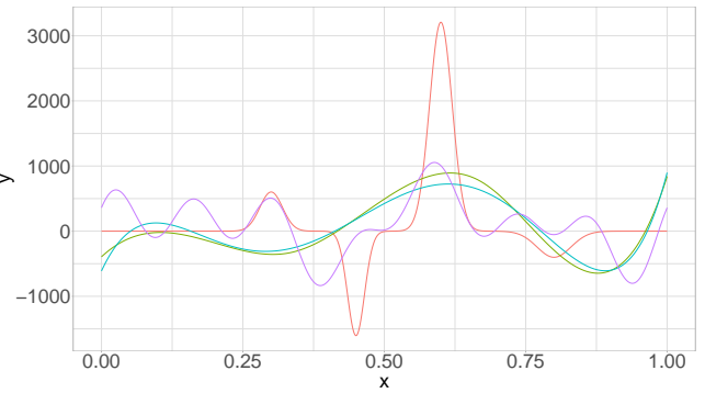
Figure 20: FPC Regression, 3 harmonics - f_2, Y_2
