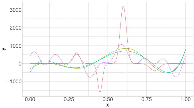
Figure 19: FPC Regression, 3 harmonics - f_2, Y_1
