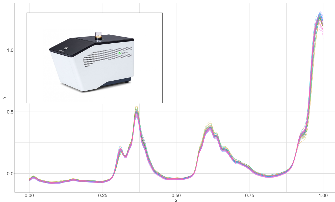
Figure 4: NIR absorption spectra from the Gasoline Data Set and Finder SD (a Near-Infrared-Spectroscopie built by HiperScan GmbH)
