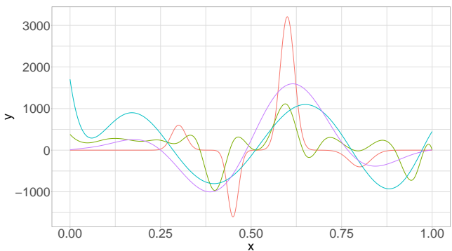
Figure 23: FPC Regression, 4 harmonics - f_2, Y_1
