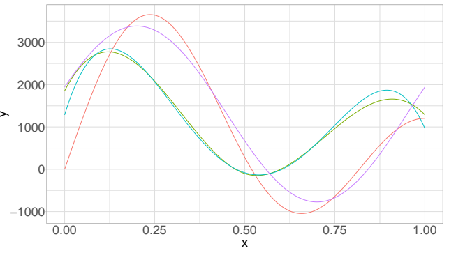
Figure 18: FPC Regression, 3 harmonics - f_1, Y_2
